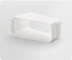
KIT0121002 15° 227×138×94mm
